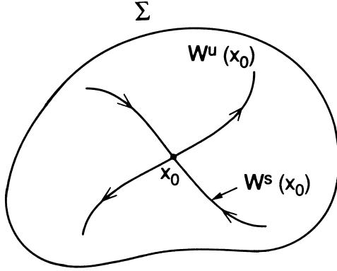
FIGURE 10.1.2. The geometry of the Poincaré map
