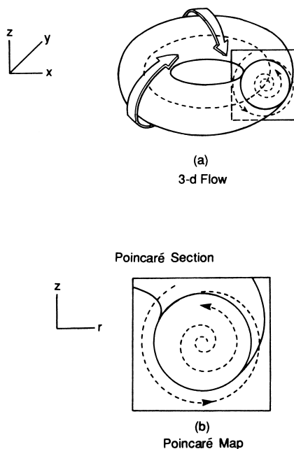
FIGURE 20.7.19. a) Three-dimensional flow, b) Poincaré section.
