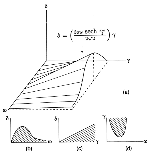
FIGURE 28.5.2. a) Graph of the critical surface \delta = \left( \frac{3\pi\omega \operatorname{sech}(\pi\omega/2)}{2\sqrt{2}} \right) \gamma . b) Cross-section of the critical surface for \gamma = \text{constant} . c) Cross-section of the critical surface for \omega = \text{constant} . d) Cross-section of the critical surface for \delta = \text{constant} .
