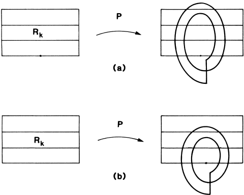
FIGURE 27.3.5. Two possibilities for P(R_k) \cap R_k .
