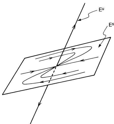
FIGURE 3.1.2. The geometry of E^s and E^u for Example 3.1.2 (for \omega < 0 ).
