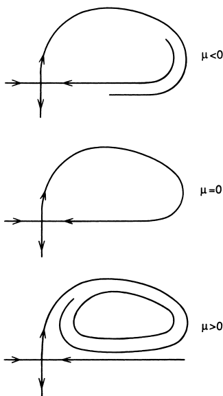
FIGURE 10.3.3. Graph of P for \mu > 0 , \mu = 0 , and \mu < 0 with \delta > 1 .
