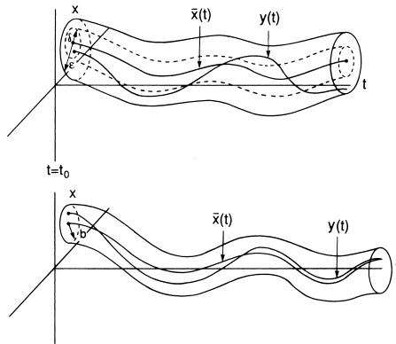
FIGURE 1.2.1. a) Liapunov stability. b) Asymptotic stability.
