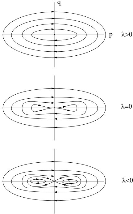
FIGURE 20.9.2. Phase portraits corresponding to the Hamiltonian pitchfork bifurcation.
