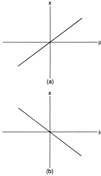
FIGURE 21.1.5. a) \left(-\frac{\partial^2 f}{\partial x^2}(0,0)/\frac{\partial^2 f}{\partial x \partial \mu}(0,0)\right) > 0 ; b) \left(-\frac{\partial^2 f}{\partial x^2}(0,0)/\frac{\partial^2 f}{\partial x \partial \mu}(0,0)\right) < 0 .
