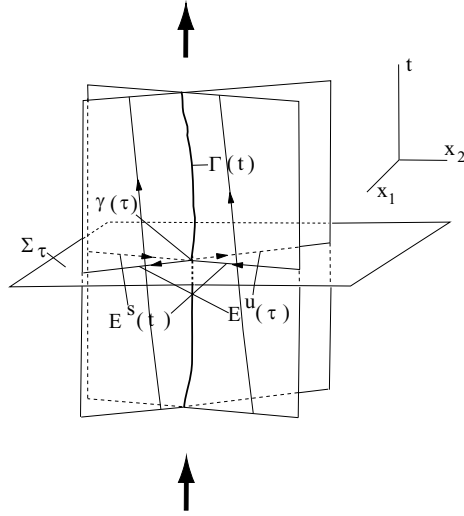
FIGURE 3.6.1. Geometry of the stable and unstable subspaces of the linearized system associated with the hyperbolic trajectory, both in the extended phase space and on a time slice, n = 2 , k = 1 . (The arrows are meant to indicate that the structure extends for all time.)
