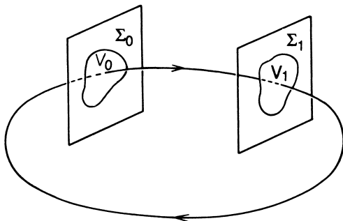
FIGURE 11.1.1. The cross-sections \Sigma_0 and \Sigma_1 .
