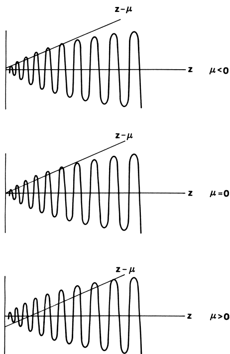
FIGURE 27.3.7. Graphical construction of the solutions of (27.3.27) for \delta < 1 .
