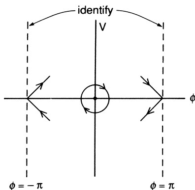
FIGURE 5.1.6. Fixed points of the pendulum.
