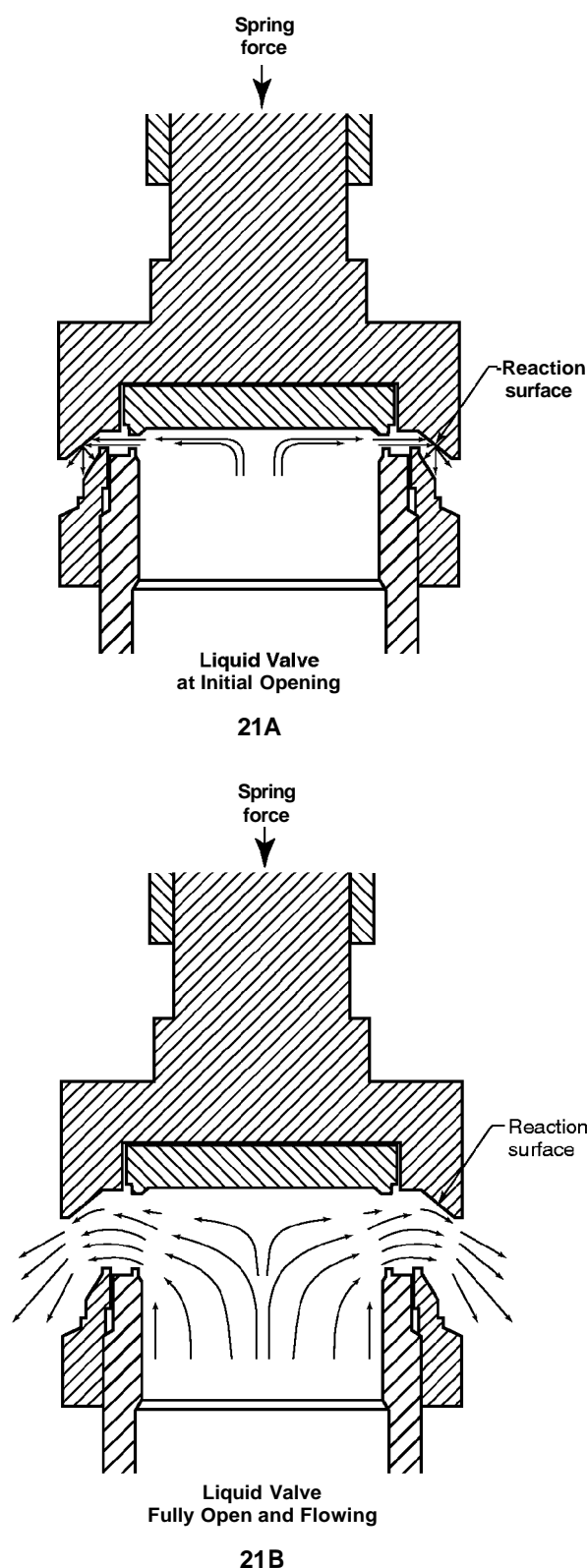
Figure 21—Pressure Relief Valve Operation—Liquid Service
