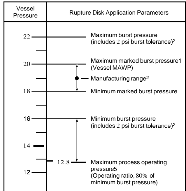
C. Example of a rupture disk with a specified burst pressure of 20 psig, manufacturing range of +0/-10%, burst tolerance of ±2 psi, and an 80% operating ratio.
