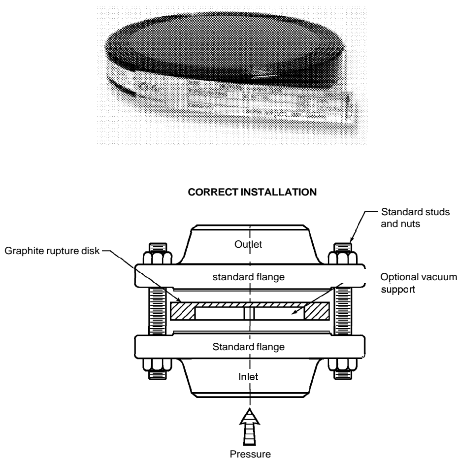
Figure 16—Graphite Rupture Disk
