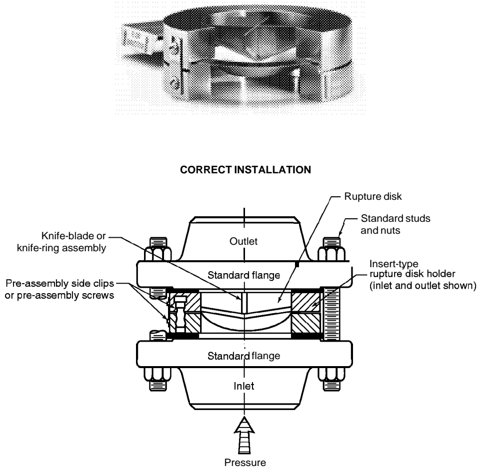
Figure 14--Reverse-Acting Rupture Disk with Knife Blades
