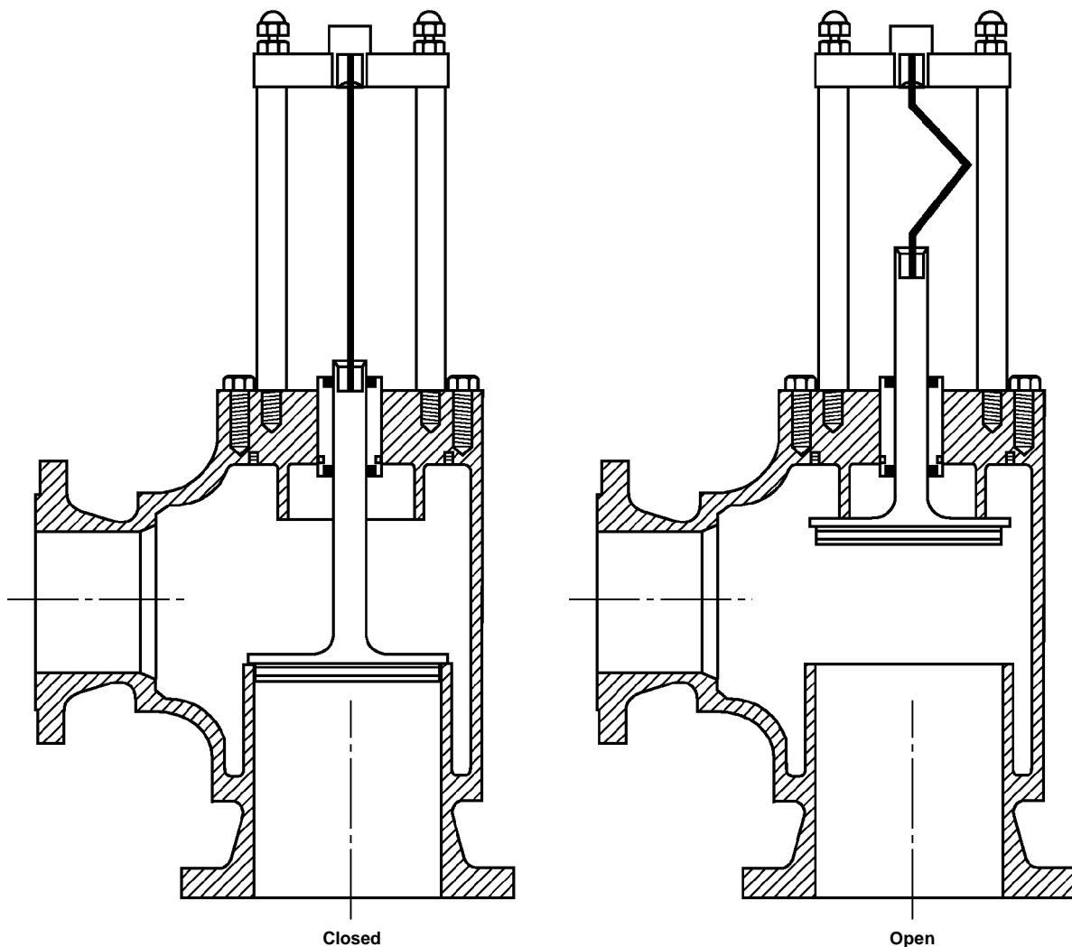
Figure 18—Buckling Pin Valve
