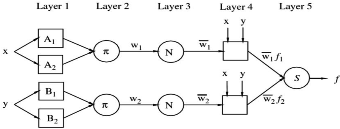
Fig.2. An ANFIS network structure for a simple FIS.
